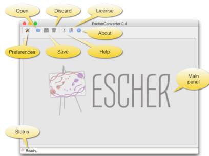
Figure 1 | The graphical user interface of EscherConverter.
